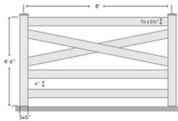
Farmington Double Cross Buck
