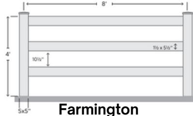
Farmington Three Rail
