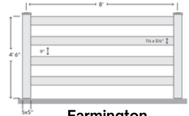
Farmington Four Rail
